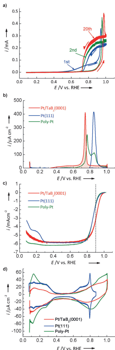
Figure 2. a) Cyclic voltammogram (CV) at 50 \text{ mVs}^{-1} for \text{Pt}/\text{TaB}_2(0001) during CO annealing. b) CV for CO stripping, as obtained by subtracting the second-cycle CV from the first-cycle CV profile. c) ORR currents measured for \text{Pt}/\text{TaB}_2(0001) , \text{Pt}(111) , and polycrystalline Pt (poly-Pt) under oxygen-saturated conditions by linear sweep voltammetry at 10 \text{ mVs}^{-1} and 1600 rpm. d) CVs measured under argon-saturated conditions for \text{Pt}/\text{TaB}_2(0001) , \text{Pt}(111) , and polycrystalline Pt after ORR evaluation.
